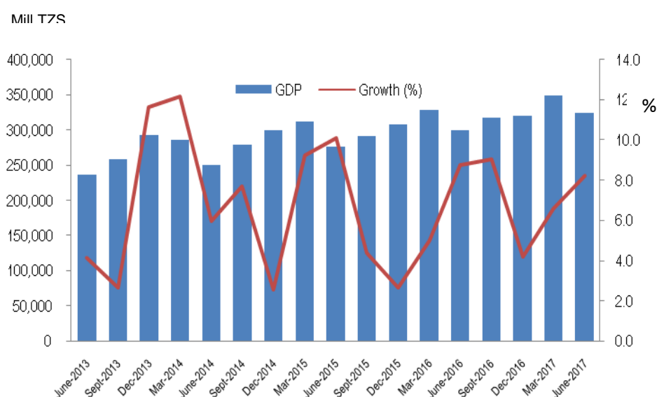
Chart 1: Total GDP at constant 2007 prices & Growth in quarterly GDP (at 2007 prices)
