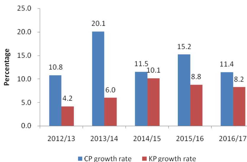
Chart 4: Percentage change in Current and Constant Prices for the year ended June (2012/13—2016/17)
